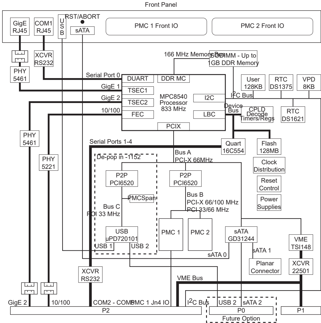
Figure 1-1 Block Diagram
