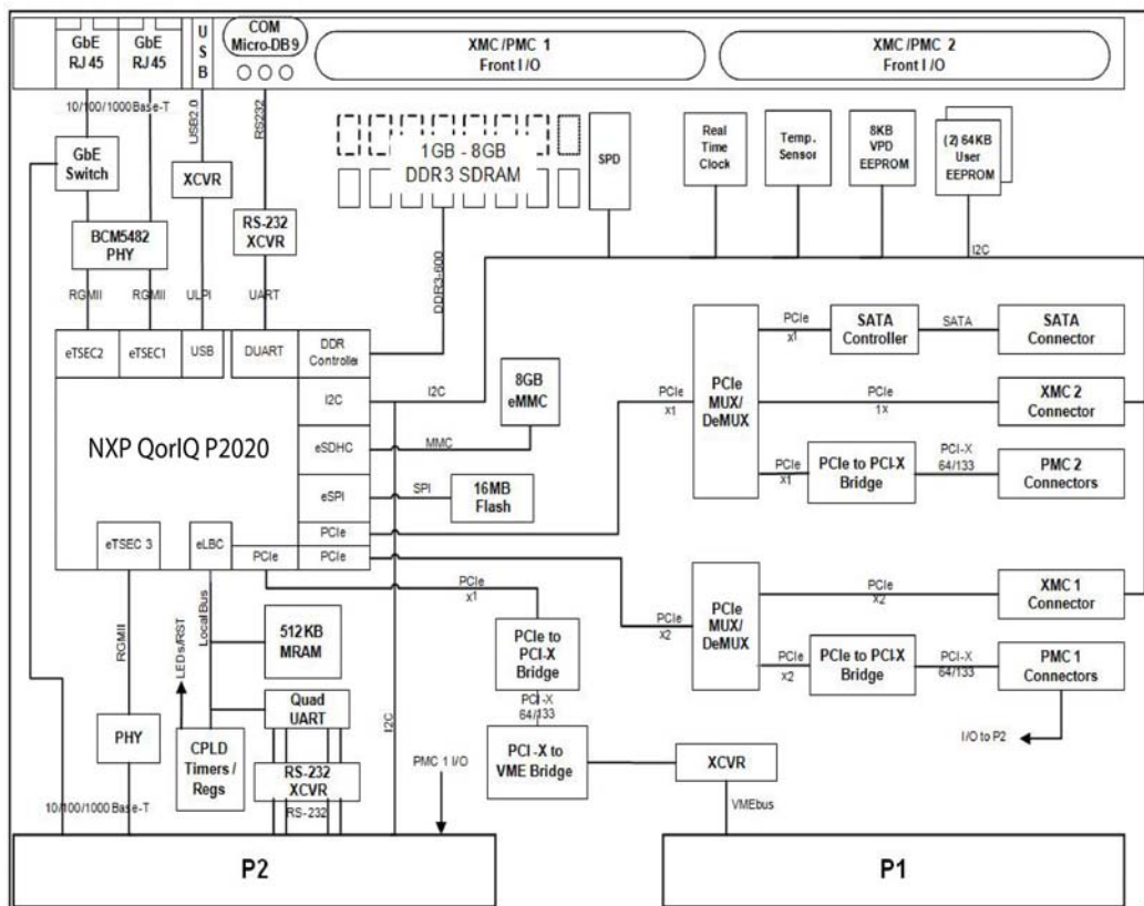
Figure 4-1 Block Diagram
