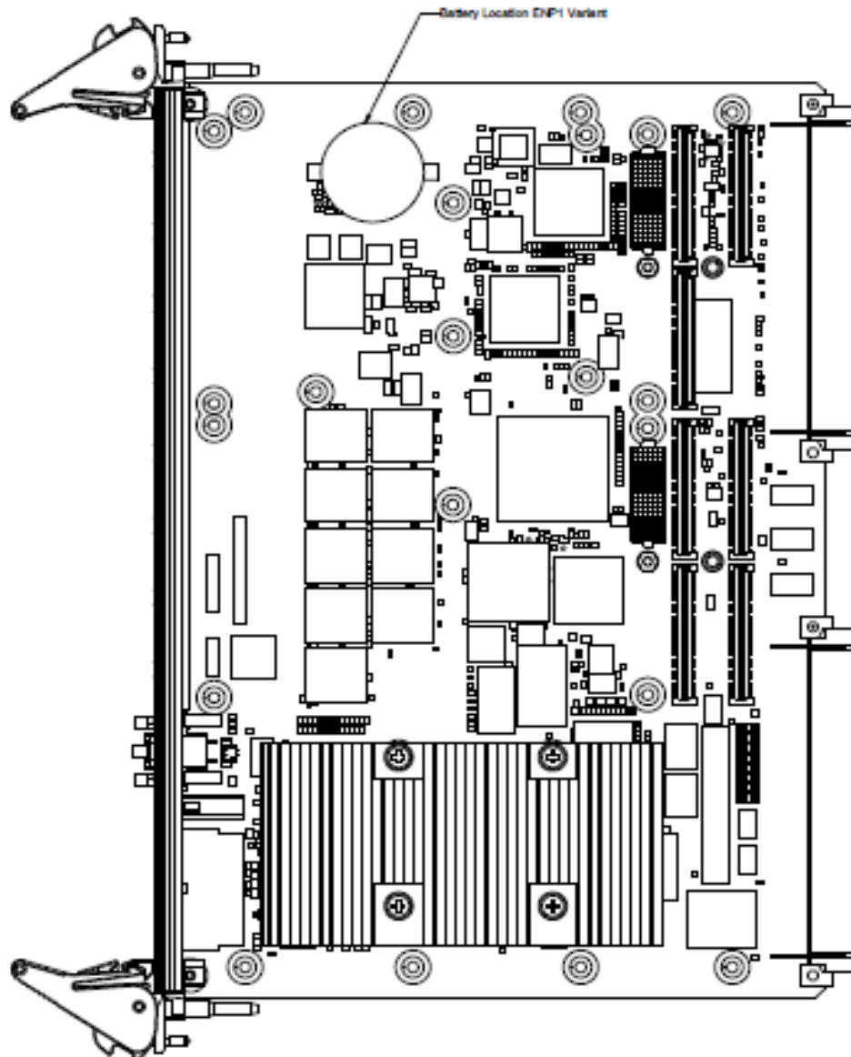
Figure A-1 Battery Location ENP1 Variant
