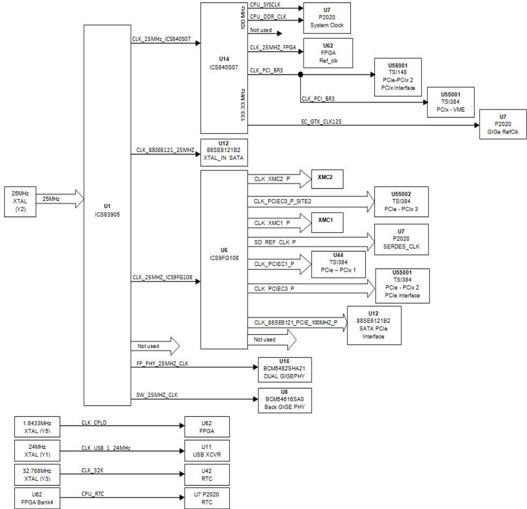
Figure 4-3 Clock Distribution Diagram
