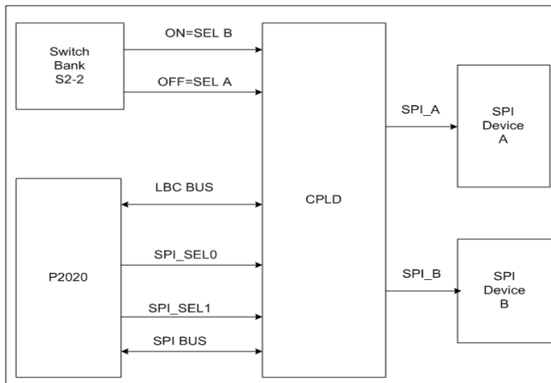
Figure 4-2 SPI Device Multiplexing Logic
