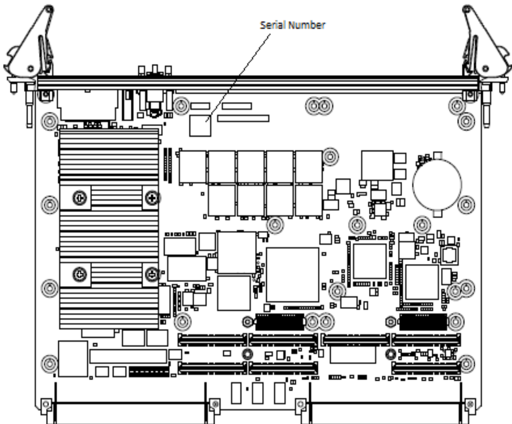
Figure 1-1 Serial Number Location-ENP1 Variant
