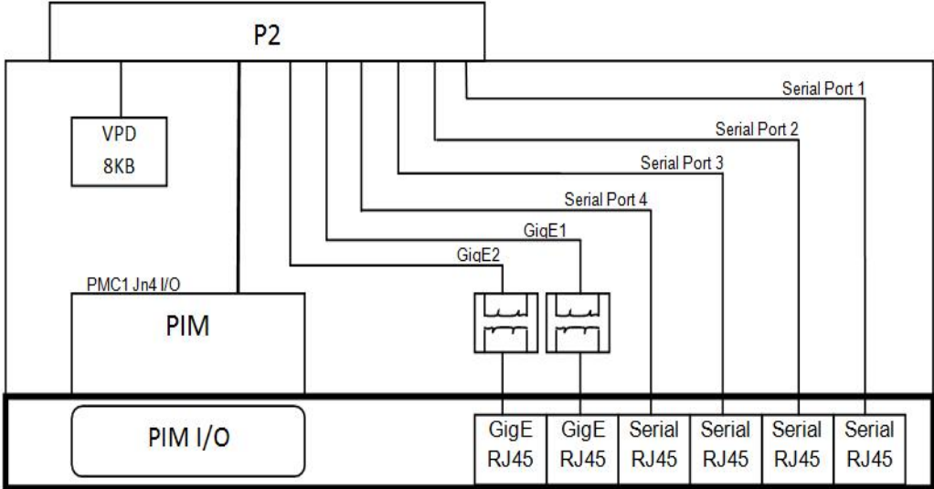
Figure 4-5 RTM Block Diagram
