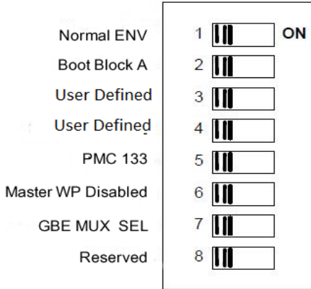
Figure 3-7 SMT Configuration Switch Position
