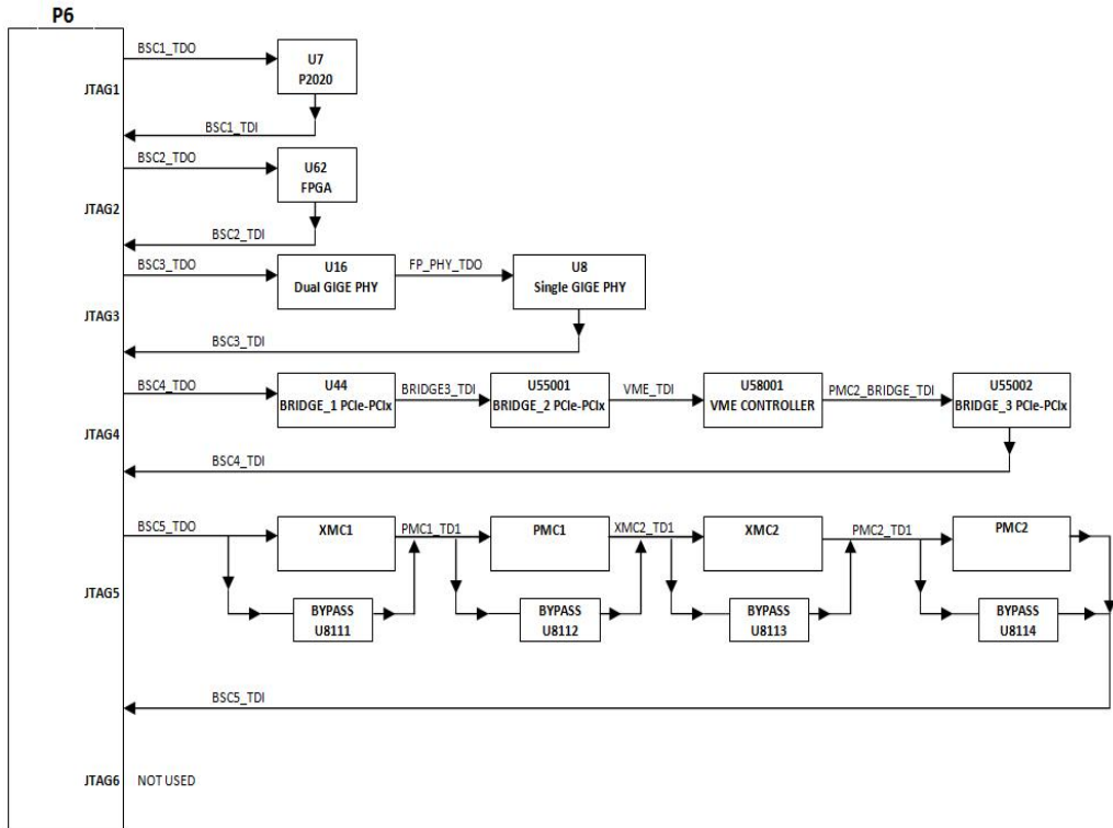
Figure 4-4 JTAG Chain Diagram
