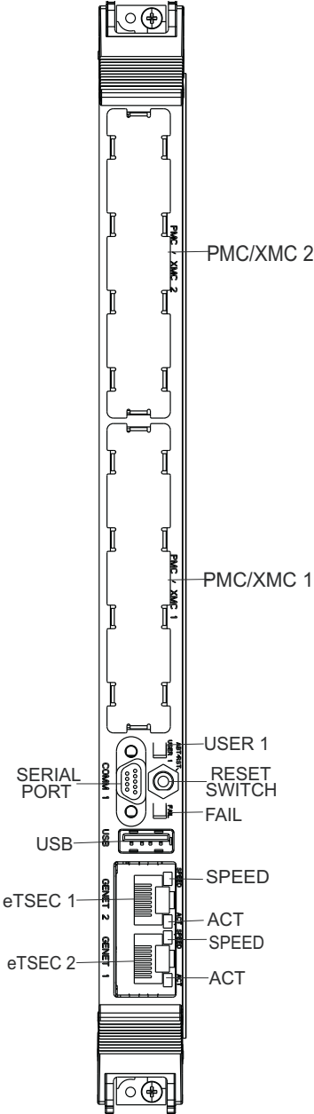
Figure 3-3 Front Panel LEDs, Connectors and Switches
